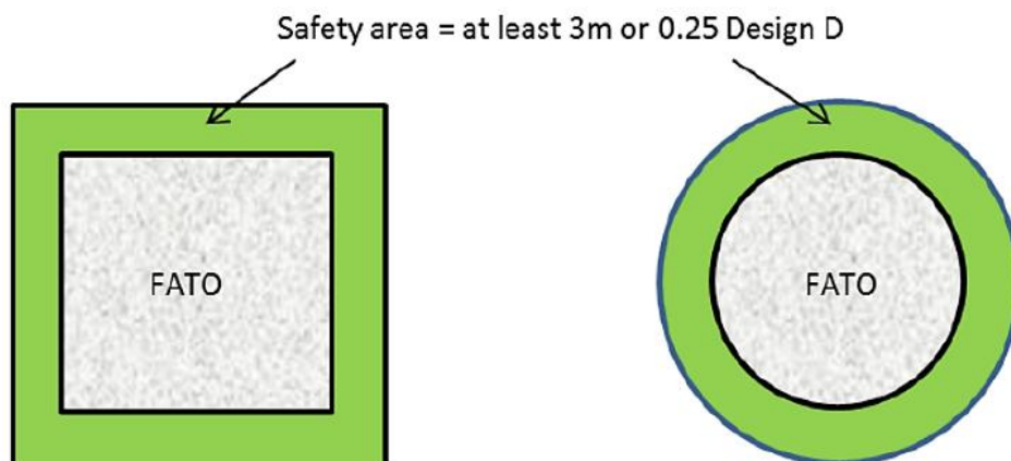
Figure 3-1. FATO and associated safety area
