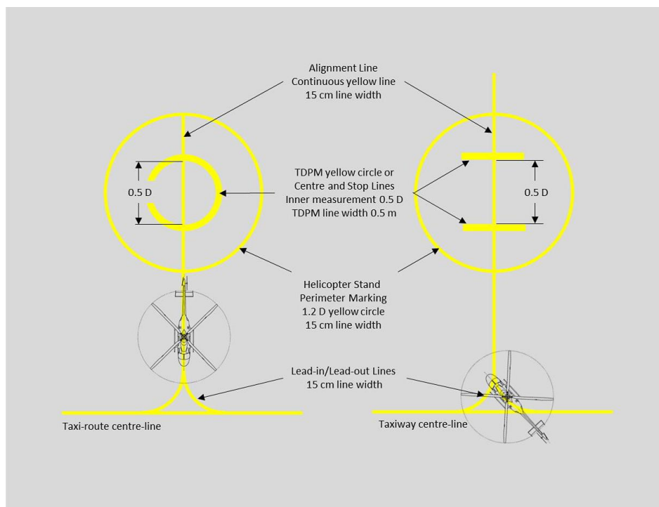
Figure 5-9. Helicopter stand markings
