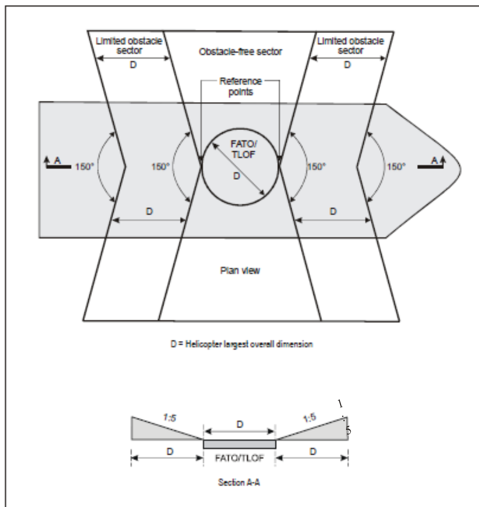
Figure 4-5. Amidship's location — Shipboard heliport obstacle limitation surfaces
