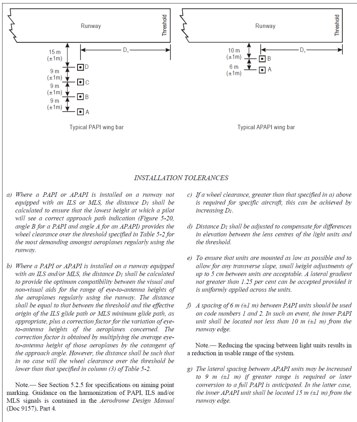
Figure 5-19. Siting of PAPI and APAPI
