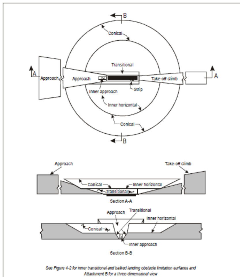
Figure 4-1. Obstacle limitation surfaces
