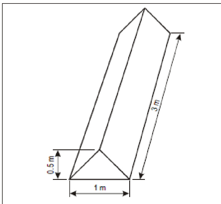
Figure 5-34. Boundary markers
