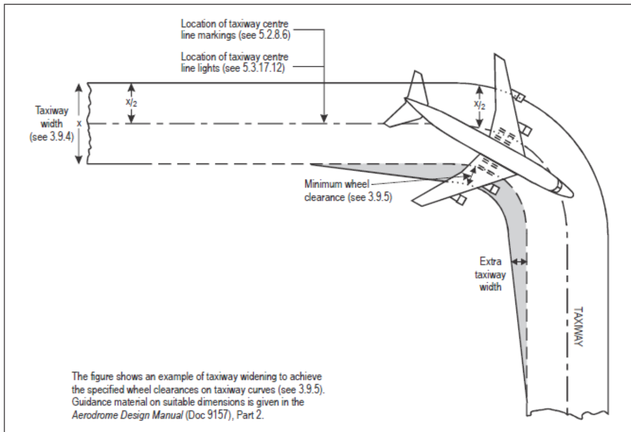
Figure 3-2. Taxiway curve
