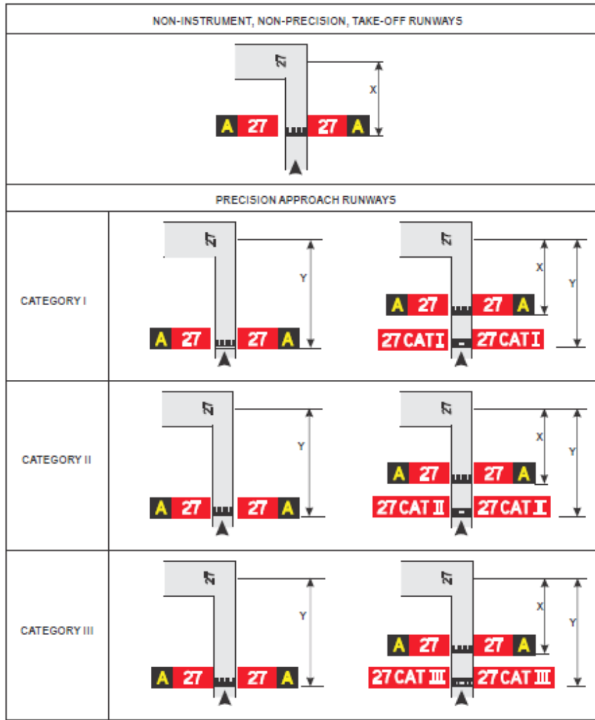
Figure 5-32. Examples of sign positions at taxiway/runway intersections
