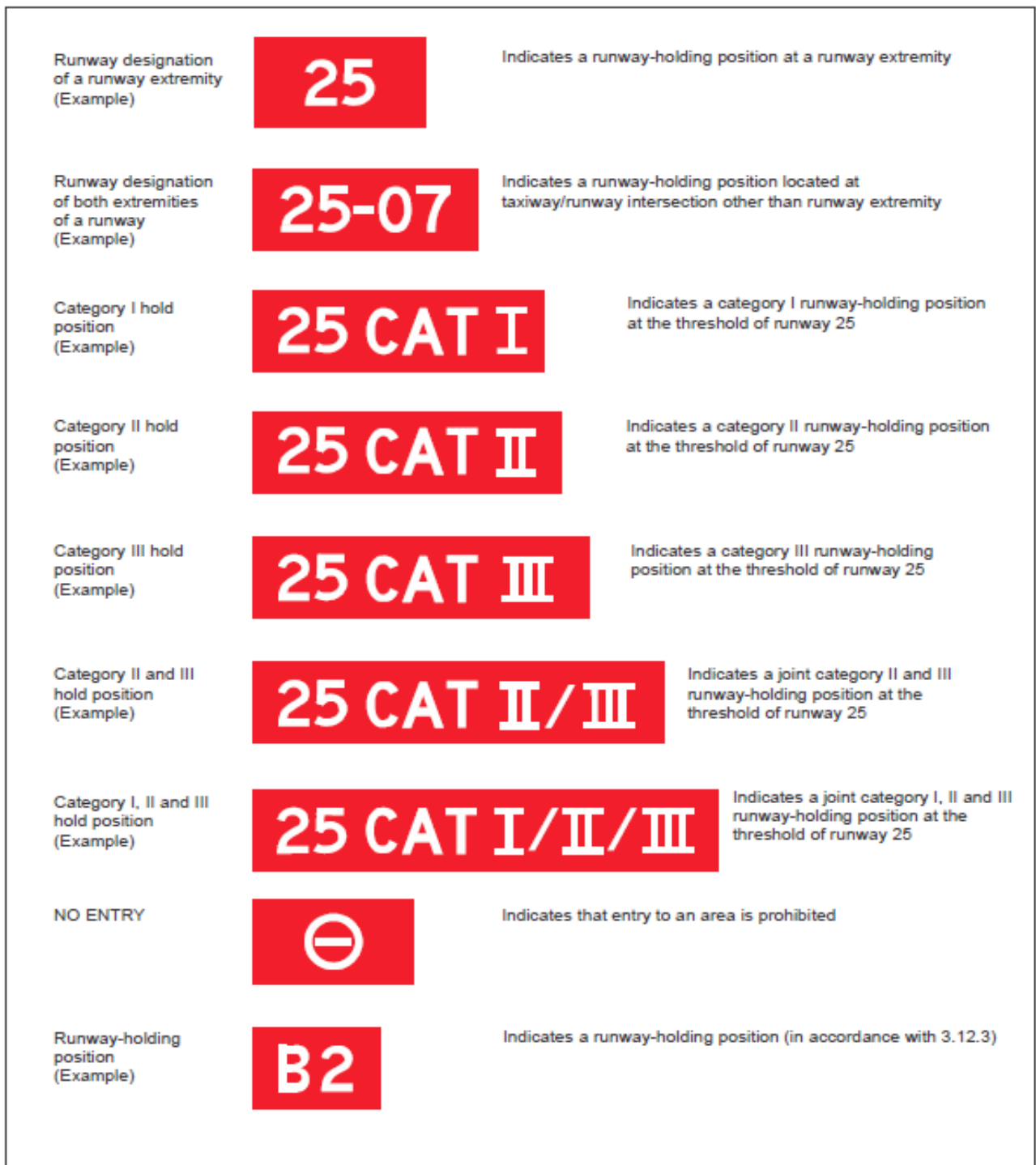
Figure 5-30. Mandatory instruction signs
